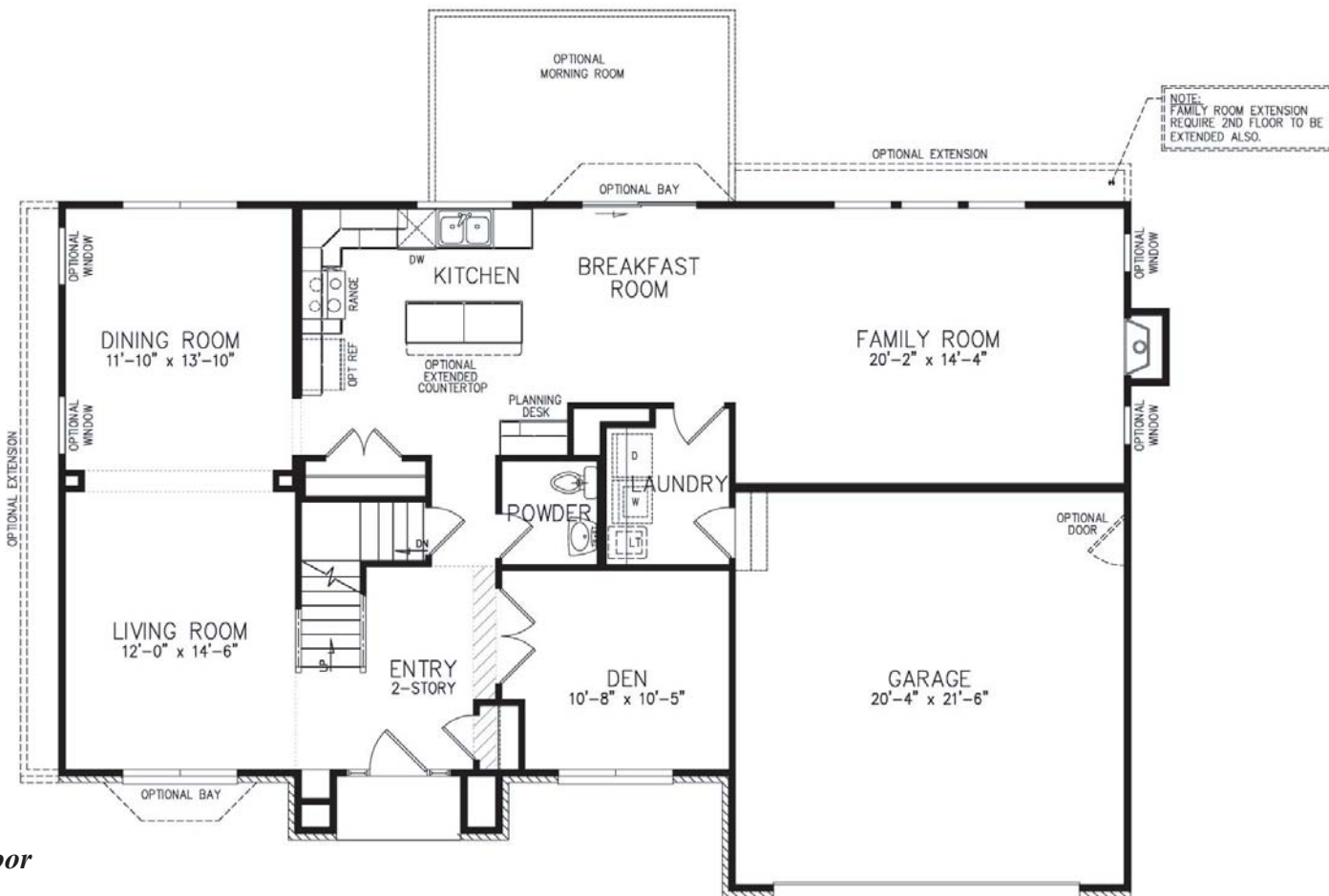
Floor plan shown with elevation A
